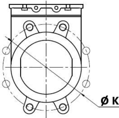
DN 400
