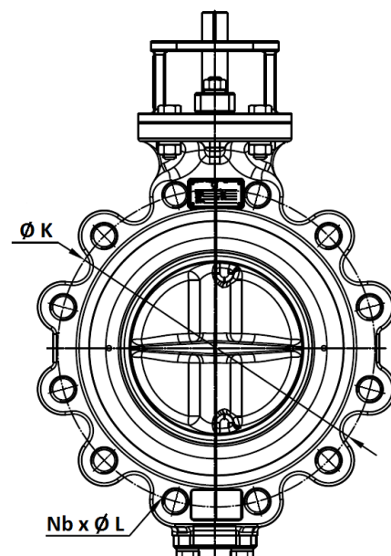
DN200 - 250
