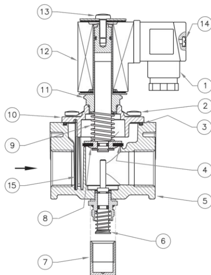
M14/RM 500 mbar – Aluminium body
